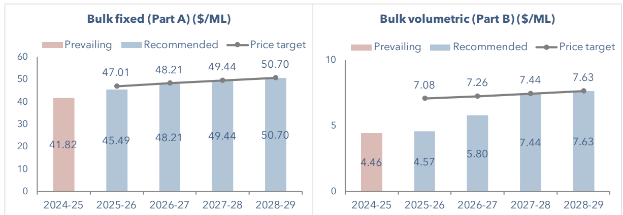
Figure 3: Draft recommended prices – Upper Burnett – John Goleby Weir ($/ML)
